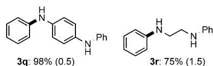
Scheme 4. Scope of the palladium-catalyzed amination of aryl mesylates. Reaction conditions: 0.6–1.0 mmol ArOMs, 1.1–5 equiv amine, [Pd]/L = 2:3, [ArOMs] = 0.25–0.1 M. See the Supporting Information. Yields are of isolated material, and mol % [\text{Pd}(\text{cinnamyl})\text{Cl}]_2 indicated within parentheses. [a] Yield determined on the basis of calibrated GC data of 3a , 3d , 3f , and 3k using dodecane as an internal standard.
