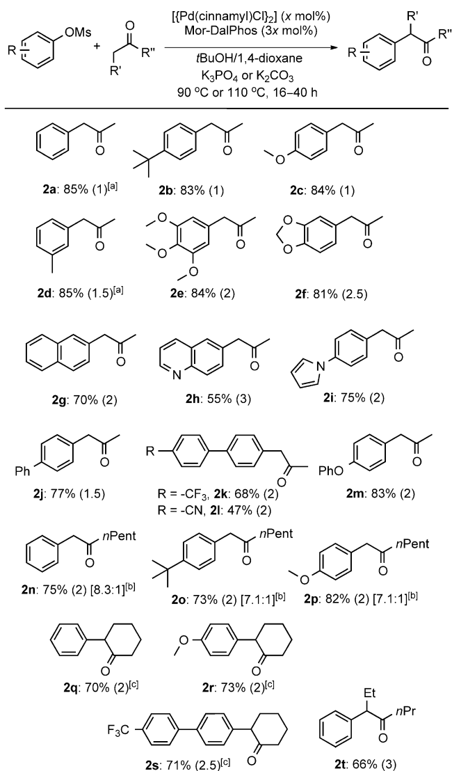
Scheme 3. Scope of the palladium-catalyzed \alpha -arylation of ketones with aryl mesylates. Reaction conditions: 0.6–0.8 mmol ArOMs, 5–10 equiv ketone, [\text{Pd}]/\text{L} = 2:3 , [\text{ArOMs}] = 0.5\text{--}0.125 M. See the Supporting Information. Yields are of isolated material, and mol% [\text{Pd}(\text{cinnamyl})\text{Cl}]_2 is indicated within parentheses. [a] Yield determined on the basis of calibrated GC data of 2a and 2d using dodecane as an internal standard. [b] Mixture of regioisomers. Ratio indicated within brackets, with major product shown. [c] Used tert -butanol solvent, \text{K}_2\text{CO}_3 , 110^\circ\text{C} .
